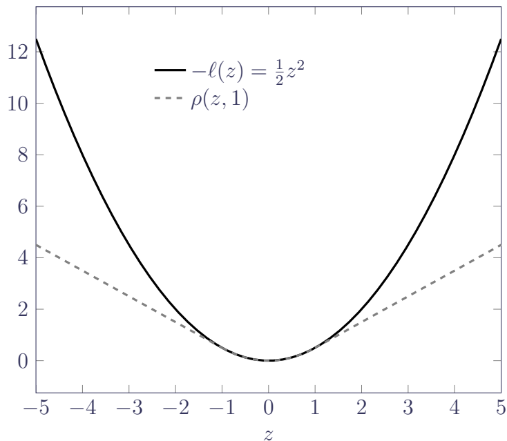
Figure 2: Contribution to (negative) log-likelihood for normal variable and robustified contribution using the Huber \rho -function of equation (2) with k = 1 .
