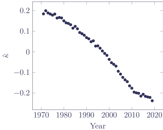
Figure 15: \hat{\kappa}_{1971+t} values from Table 4.
