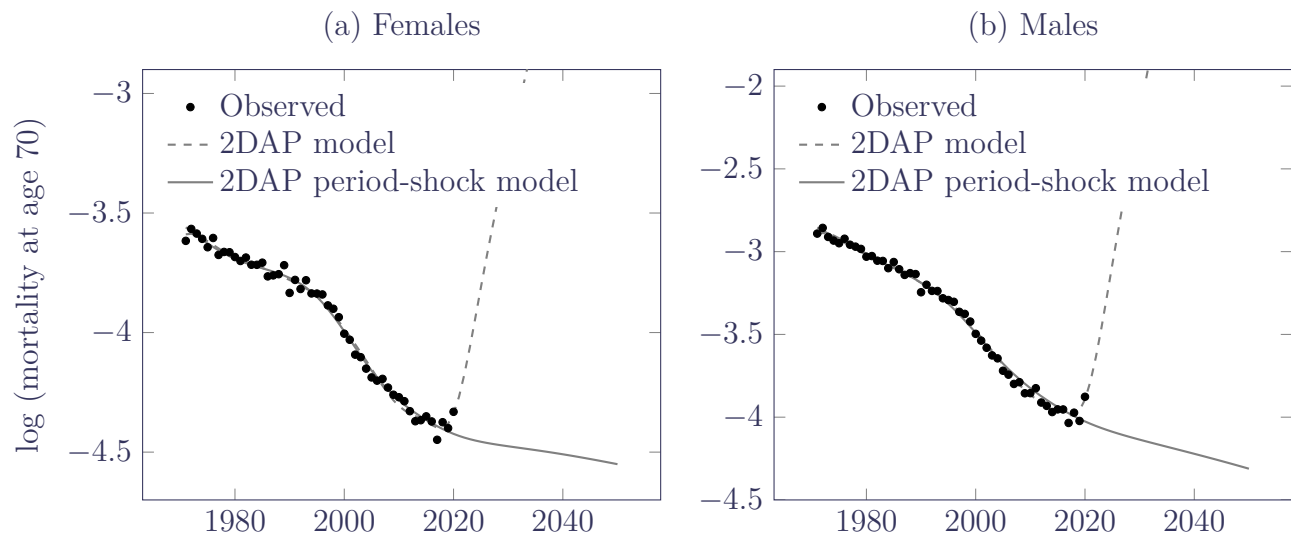
Figure 13: Observed mortality rates at age 70 with forecasts using ordinary 2DAP model [Currie et al., 2004] and 2DAP period-shock model [Kirkby and Currie, 2010]. Source: own calculations using data for males and females in England & Wales aged 50-105, over the period 1971-2020.
