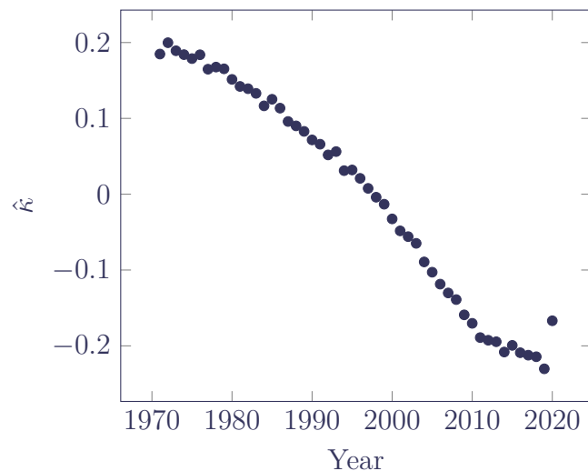
Figure 17: \hat{\kappa}_{1971+t} values from Table 5, showing the outlier in 2020.
