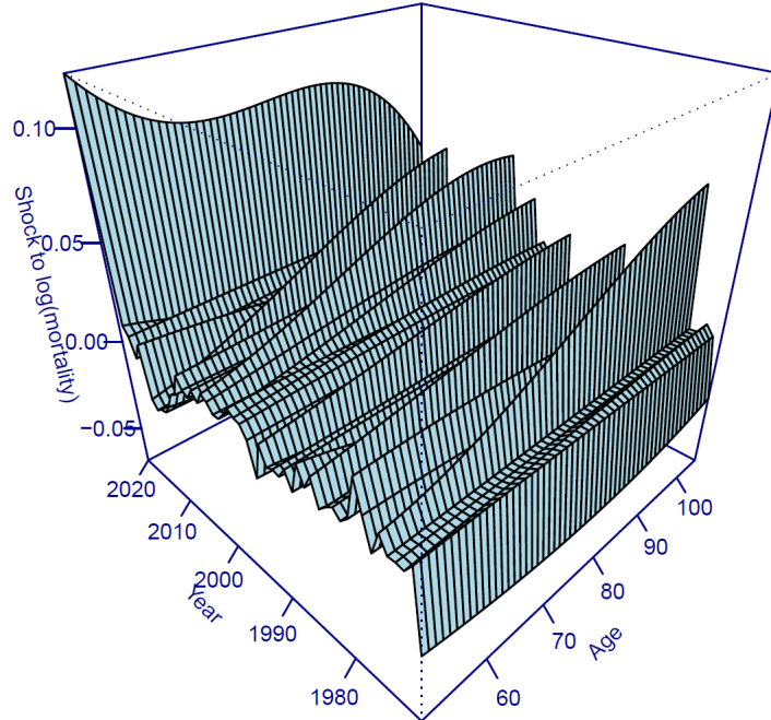
Figure 12: Period shocks under optimised scaling using equation (18). Source: own calculations using data for females in England & Wales aged 50-105, over the period 1971-2020.
