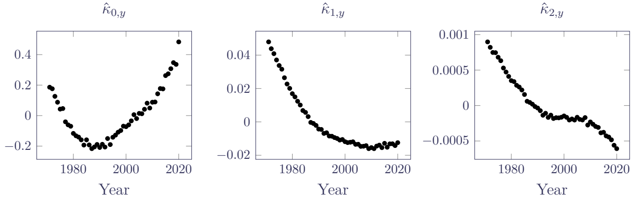
Figure 5: Estimates for period effects under minimally-constrained M9 model. These parameter estimates are not consistent with a multivariate random walk with drift. Contrast with the over-constrained equivalent in Figure 6. Source: Own calculations using HMD data, females aged 50–105, 1971–2020.
