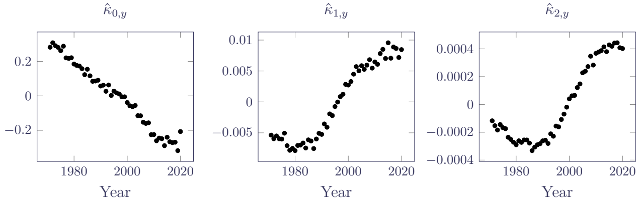
Figure 6: Estimates for forecasting parameters under over-constrained M9. Contrast with the minimally-constrained equivalent in Figure 5. Source: Own calculations using HMD data, females aged 50–105, 1971–2020.
