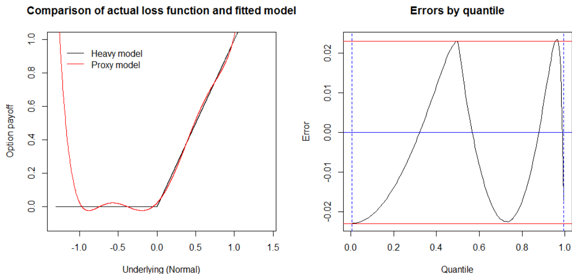
Figure 4.4: Fitting an option pay-off using minimax; note that the errors from a Normally distributed underlying are bounded between known intervals (within the fitting bounds)
