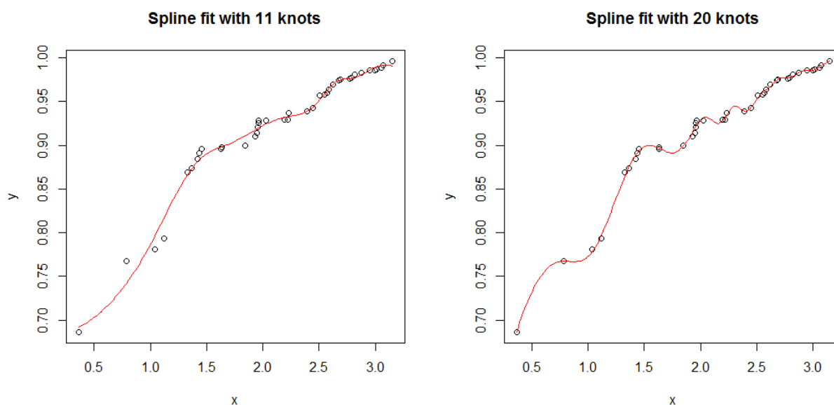
Figure 4.2: Fitting the examples above with a cubic spline basis: visually, 20 knots seems to overfit the data
