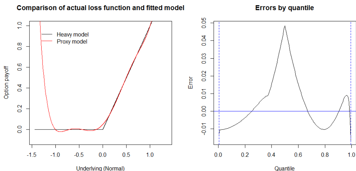
Figure 4.3: Fitting an option pay-off using least squares (left) and errors from a Normally distributed underlying (right). Note that errors explode outside of the fitting bounds and so the errors graph is bounded between the 0.5 th percentile and the 99.5 th , to keep the scale manageable, otherwise the large error at the extremely small percentiles would dominate
