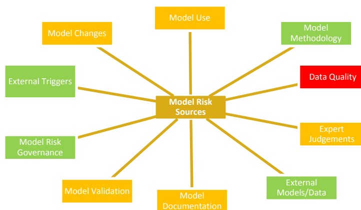
Figure 2.3: Diagrammatic presentation of qualitative model risk assessment
