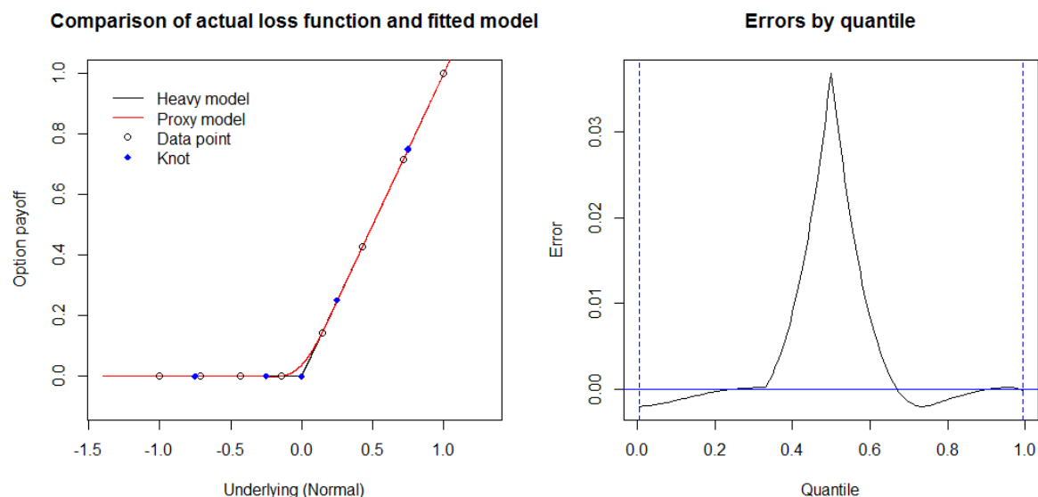
Figure 4.5: Fitting an option pay-off using regression cubic splines; note that the errors from a Normally distributed underlying are small at the extremes
